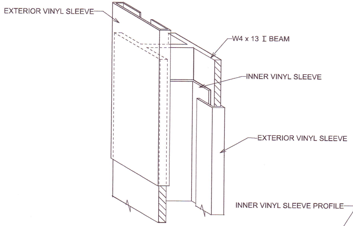
POST SLEEVE VIEW
